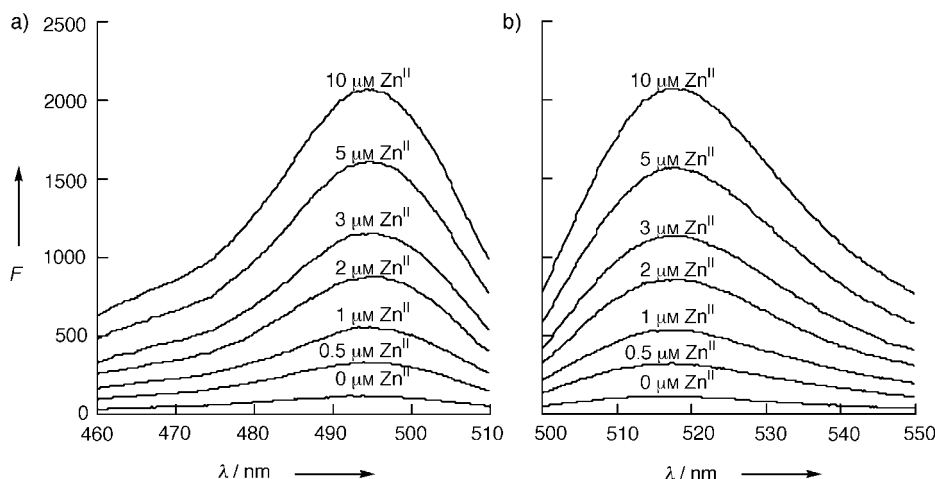
Figure 1. a) Excitation spectra (emission at \lambda_{\text{em}} = 515\text{ nm} ) and b) emission spectra (excitation at \lambda_{\text{ex}} = 495\text{ nm} ) of ACF-1 ( 5\text{ }\mu\text{M} ) in the presence of \text{Zn}^{\text{II}} from 0–10 \mu\text{M} . These spectra were measured at pH 7.5 (100 mM HEPES buffer). F = Fluorescent intensity (arbitrary units).
